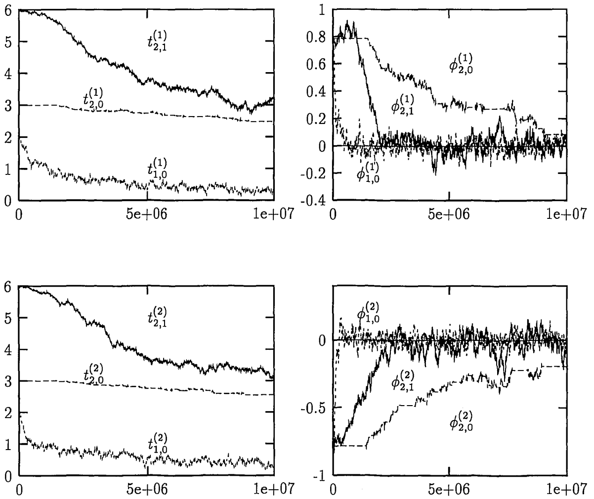
Figure 5.5: Case 1: Time evolution of the parameters for a system with two ternary sensors and generalized Gaussian noise with k = 2.0 .
